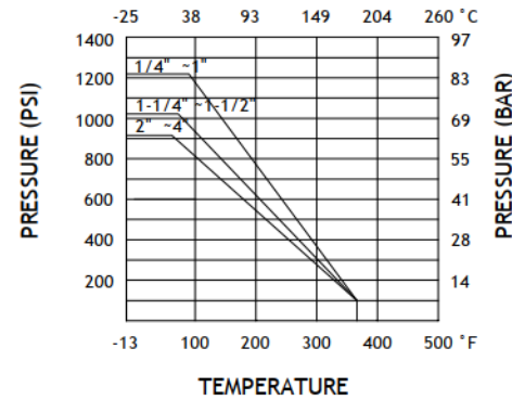
PRESSURE-TEMPERATURE RATING
